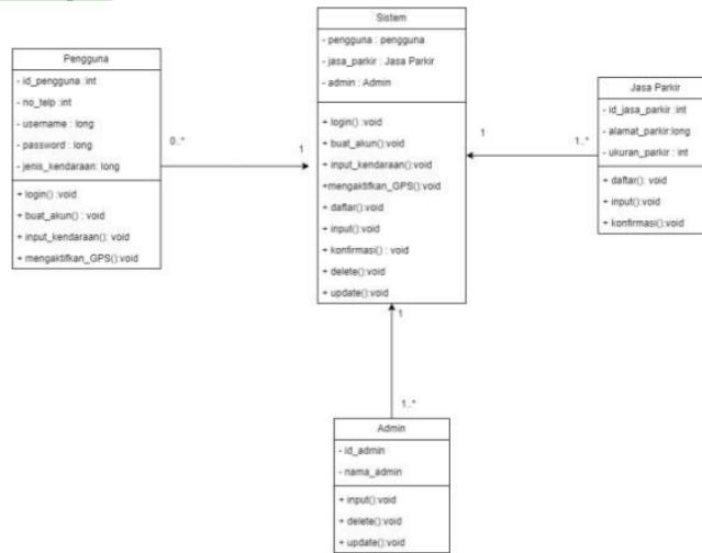
Gambar 2 Class Diagram
