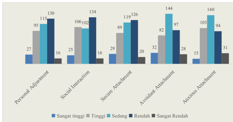
Fig. 1: Frequency Distribution
