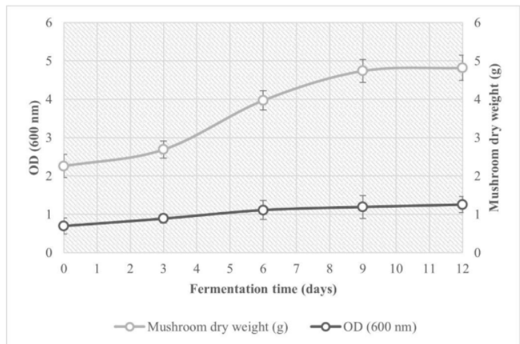
Fig. 1. Optical density (OD 600 nm) and mushrooms dry weight patterns during butterfly pea flower kombucha fermentation.
