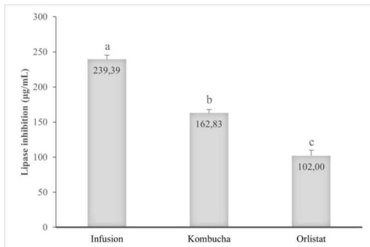
Fig. 4. Inhibitory activities ( IC_{50} ) of butterfly pea flower infusion, kombucha, and orlistat on pancreatic lipase. The data represented by distinct letters exhibit a significant difference ( P < 0.05 ). The values are presented as means \pm standard deviation.
