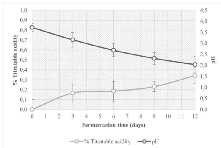
Fig. 2. Titratable acidity and pH during butterfly pea flower kombucha fermentation.
