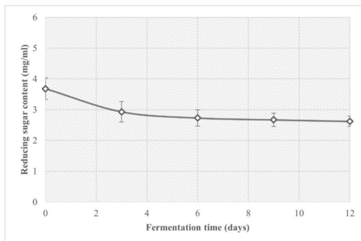
Fig. 3. Reducing sugar content during butterfly pea flower kombucha fermentation.
