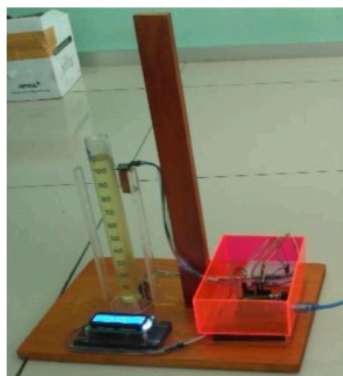
Figure 4. Apparatus for experiments on viscosity in fluids
