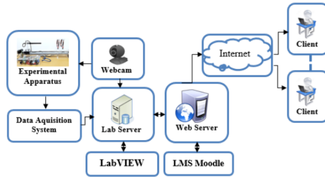
Figure 1. Remote Laboratory Hardware System Design Diagram
