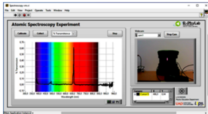
Figure 3. Remote Experiment Results of Hydrogen Atom Spectroscopy
