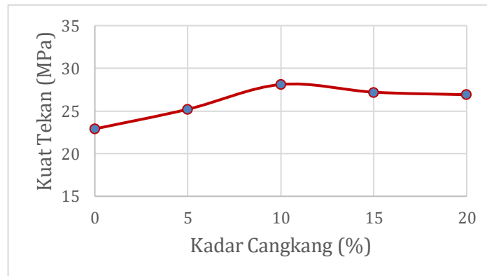
Figure 2. Comparison of Shell Content to Concrete Compressive Strength
