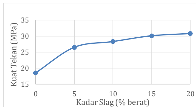
Figure 1. Comparison of Slag Content to Concrete Compressive Strength
