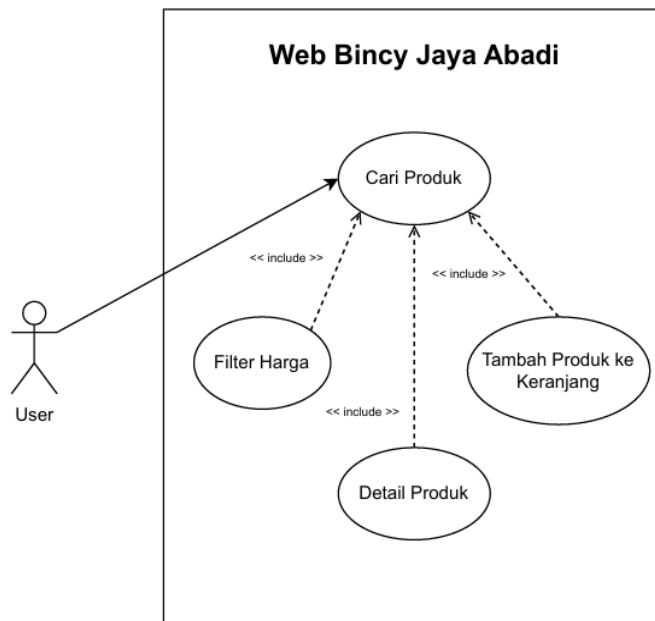
Gambar 3. 12 Use case User
