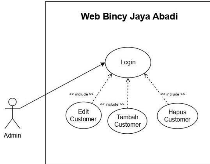
Gambar 3. 15 Use case Admin Data Costumer
