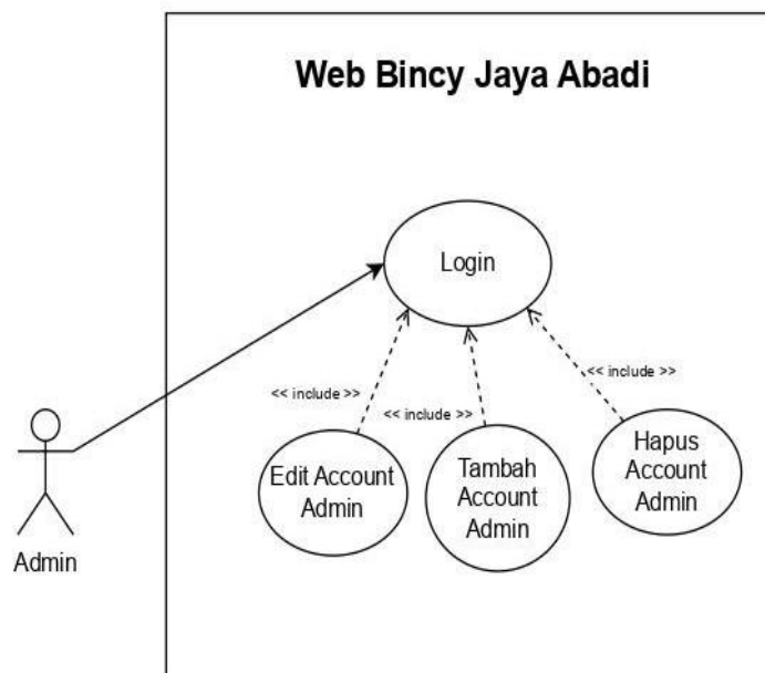
Gambar 3. 13 Use case Admin Account
