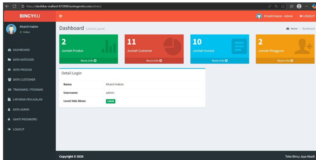
Gambar 3. 40 Dashboard Admin
