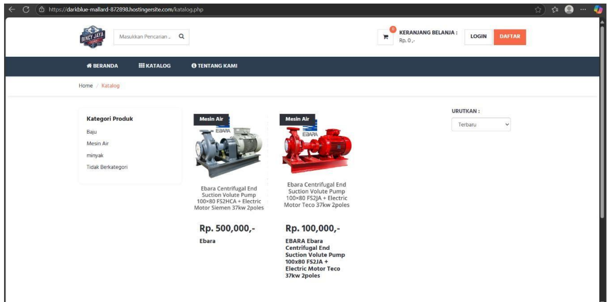
Gambar 3. 31 Halaman Katalog
