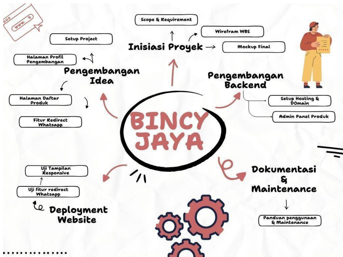
Gambar 2. 1 WBS
