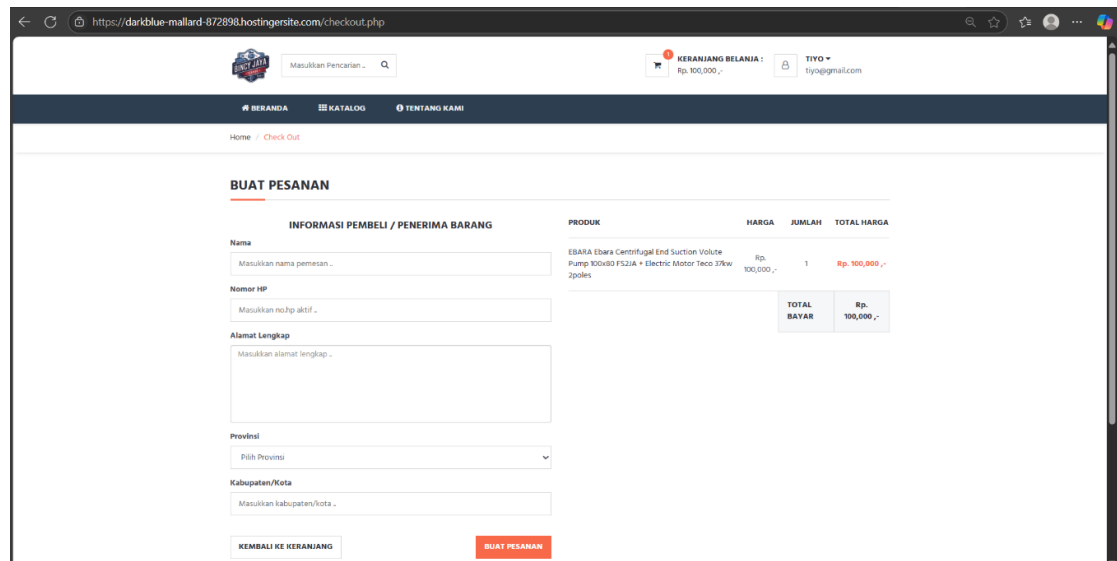
Gambar 3. 37 Halaman Checkout
