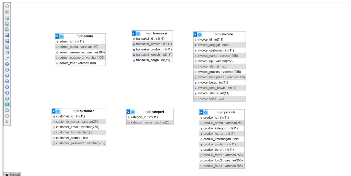
Gambar 3. 26 Database Sistem Website Bincy Jaya Abadi
