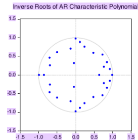
Figure 3 Inverse Roots of AR Characteristic Polynomial
